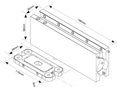
PDC100-S
