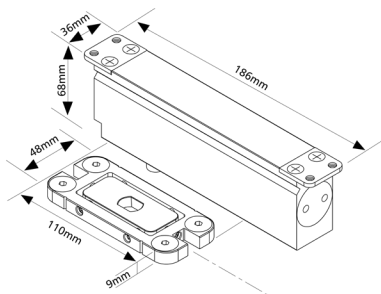
PDC100-SR
